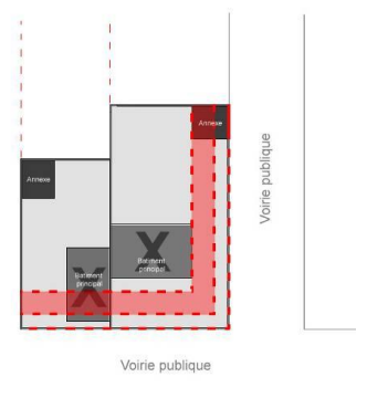
Art. UB6 – Implantations interdites
