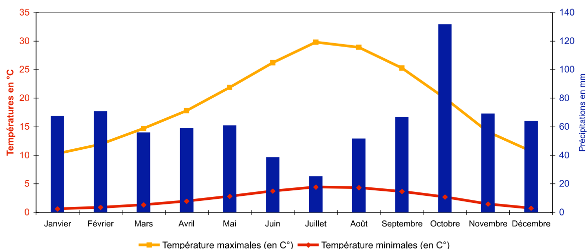
Diagramme ombrothermique (Station Nîmes)
