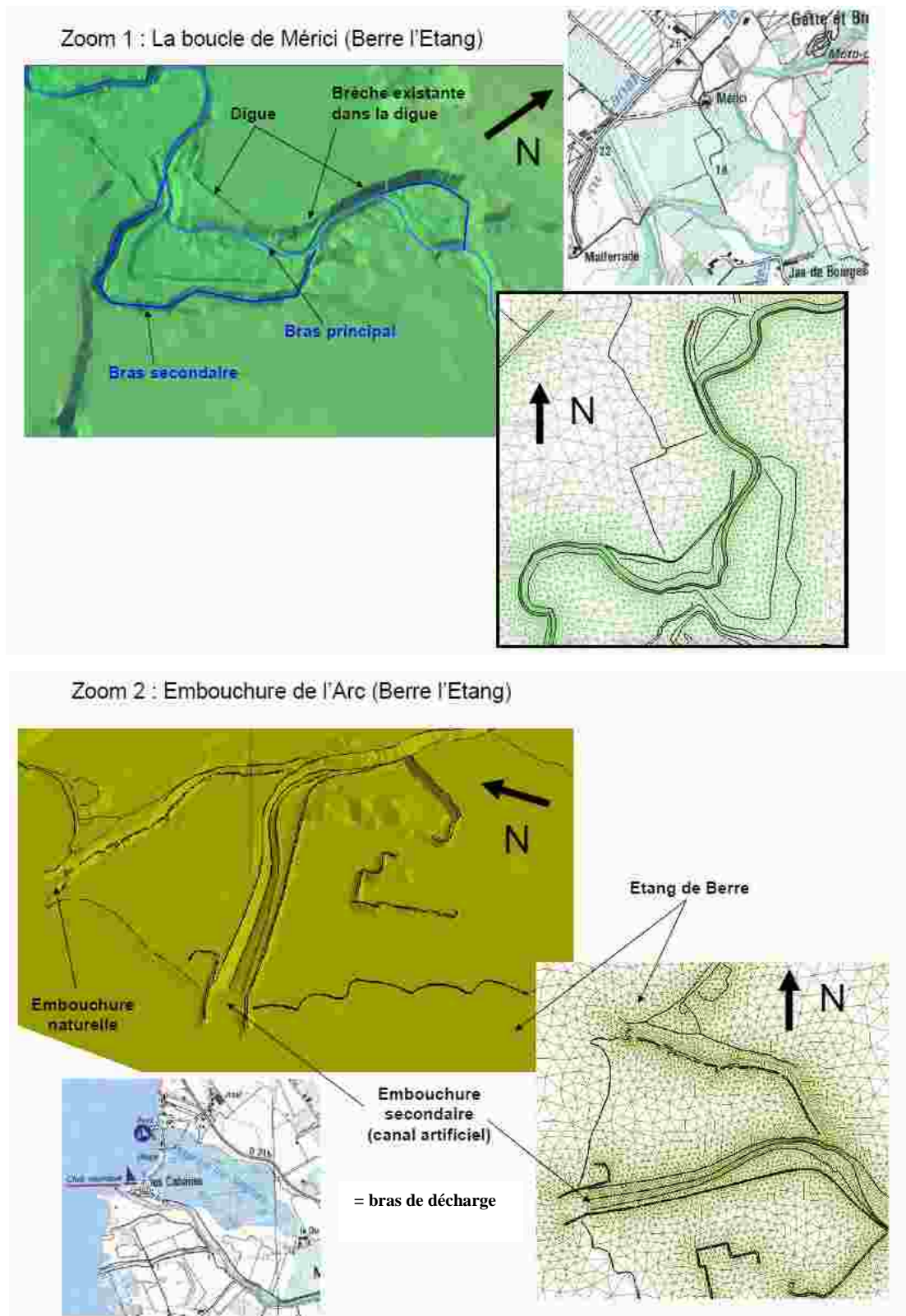
Figure 29 : maillage aval
