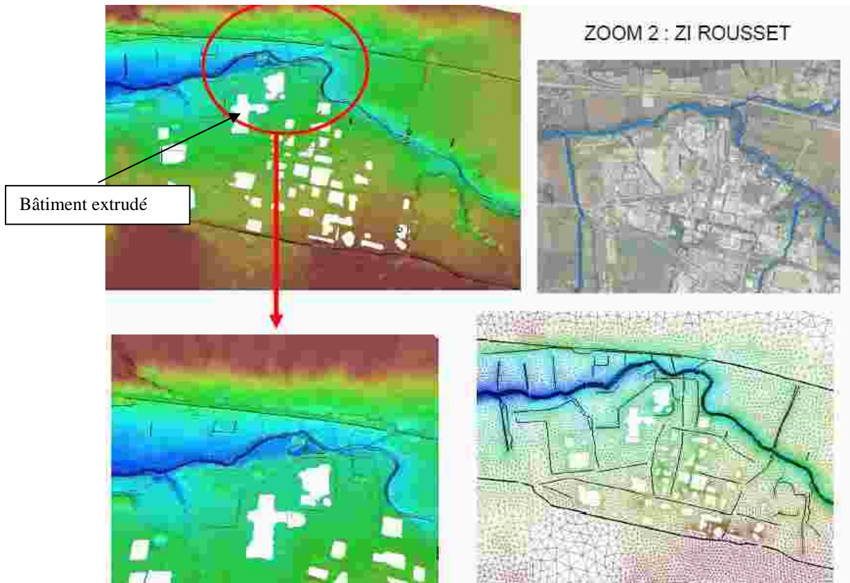
Figure 26 : maillage amont
