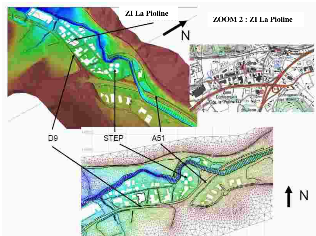
Figure 27 : maillage centre
